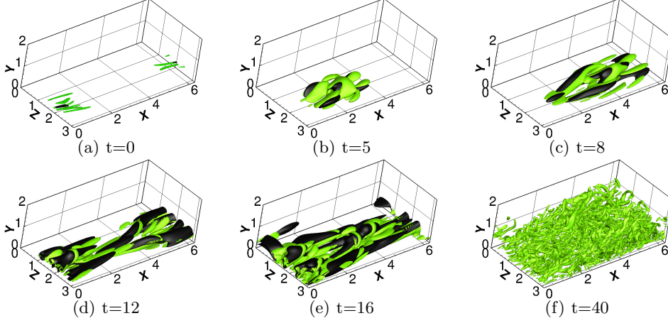
FIGURE 5. Evolution of non-linear optimal perturbation for T_{opt} = 10 and E_0 = 2 \times 10^{-6} . Iso-surface of Q-criterion ( (a-e) Q = 0.02 ; (f) Q = 0.1 , green) and streamwise velocity disturbance ( u = -0.03 , black).
