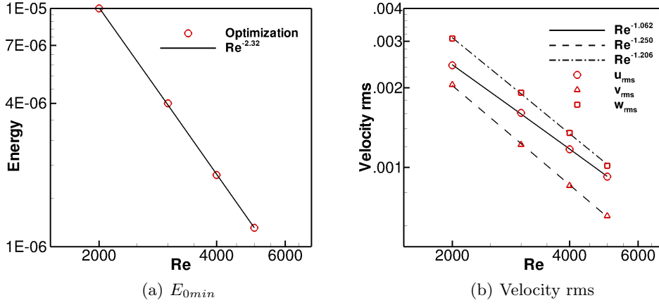
FIGURE 1. Log-Log plot indicating the scaling law for the minimal energy density (a) and velocity amplitude (b) of such an highly non-linear optimal perturbation able to suddenly provide hairpin formation in subcritical transition.
