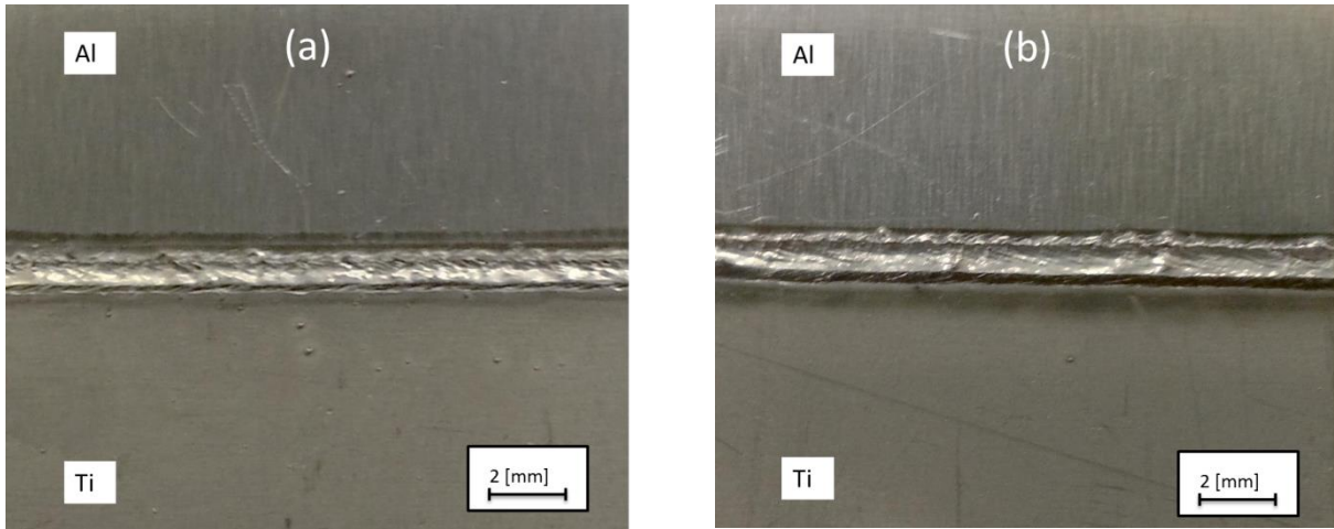
Fig. 5. Joint 6 (1.5 kW-1.8m/min-0.75mm) observed at the (a) top and (b) bottom surface.
