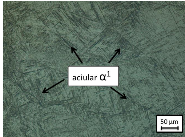
Fig. 6 Microstructure of the FZ of sample 4.
