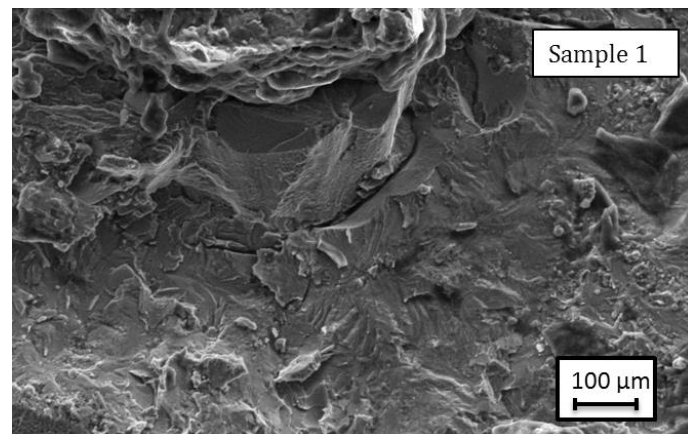
Fig. 13 Fracture surface of sample 1.
