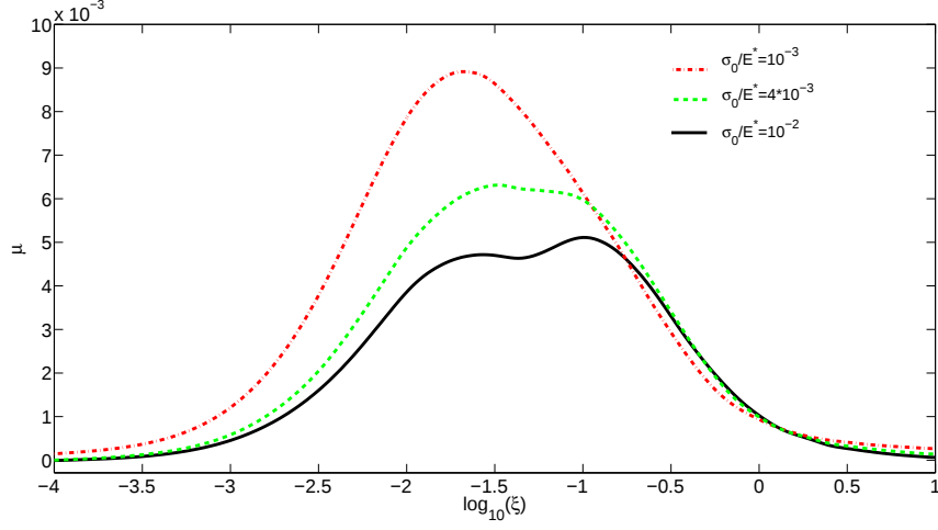
Figure 8: Viscoelastic friction coefficient \mu as a function of the dimensionless sliding speed \xi = v\tau/L for the constant thickness h/L = 0.06 and different values of the normal load \sigma_0/E^* : \sigma_0/E^* = 10^{-2} (black curve), \sigma_0/E^* = 4 \cdot 10^{-3} (green dotted curve), \sigma_0/E^* = 10^{-3} (red dotted curve).
