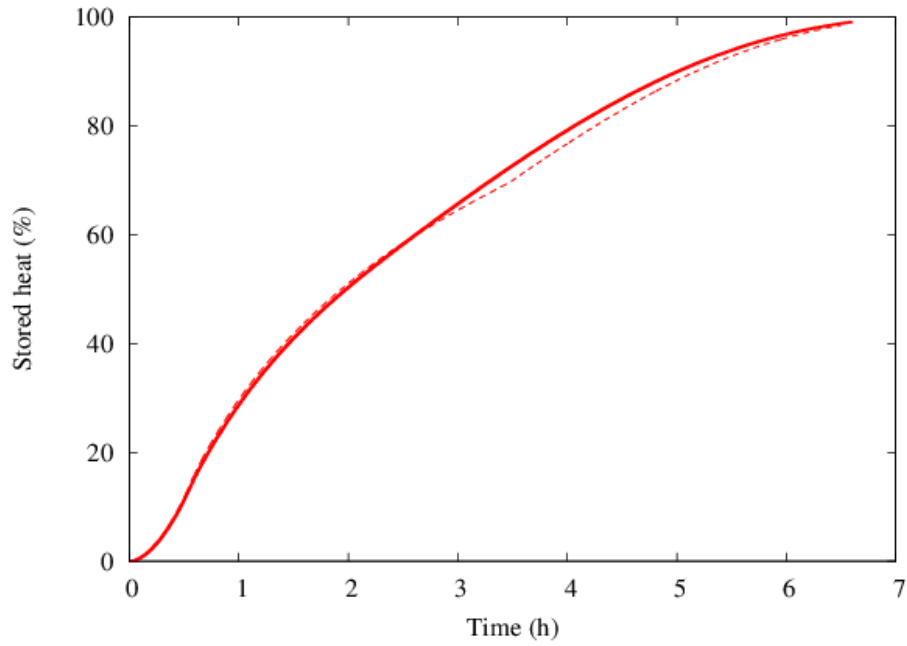
Figure 17 - Stored heat percentage. A_{mush}=1.0 \cdot 10^5 kg/(m 3 s) (continuous line),
