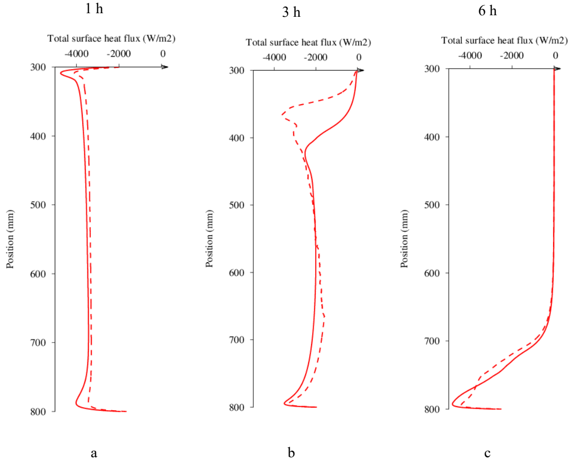
Figure 16 - Total surface heat flux along the height of the solid duct at different instants: t=1h (a), t=3h (b), t=6h (c). A_{mush}=1.0 \cdot 10^5 \text{ kg/(m}^3\text{s)} (continuous line), A_{mush}=5.0 \cdot 10^5 \text{ kg/(m}^3\text{s)} (dotted line)
