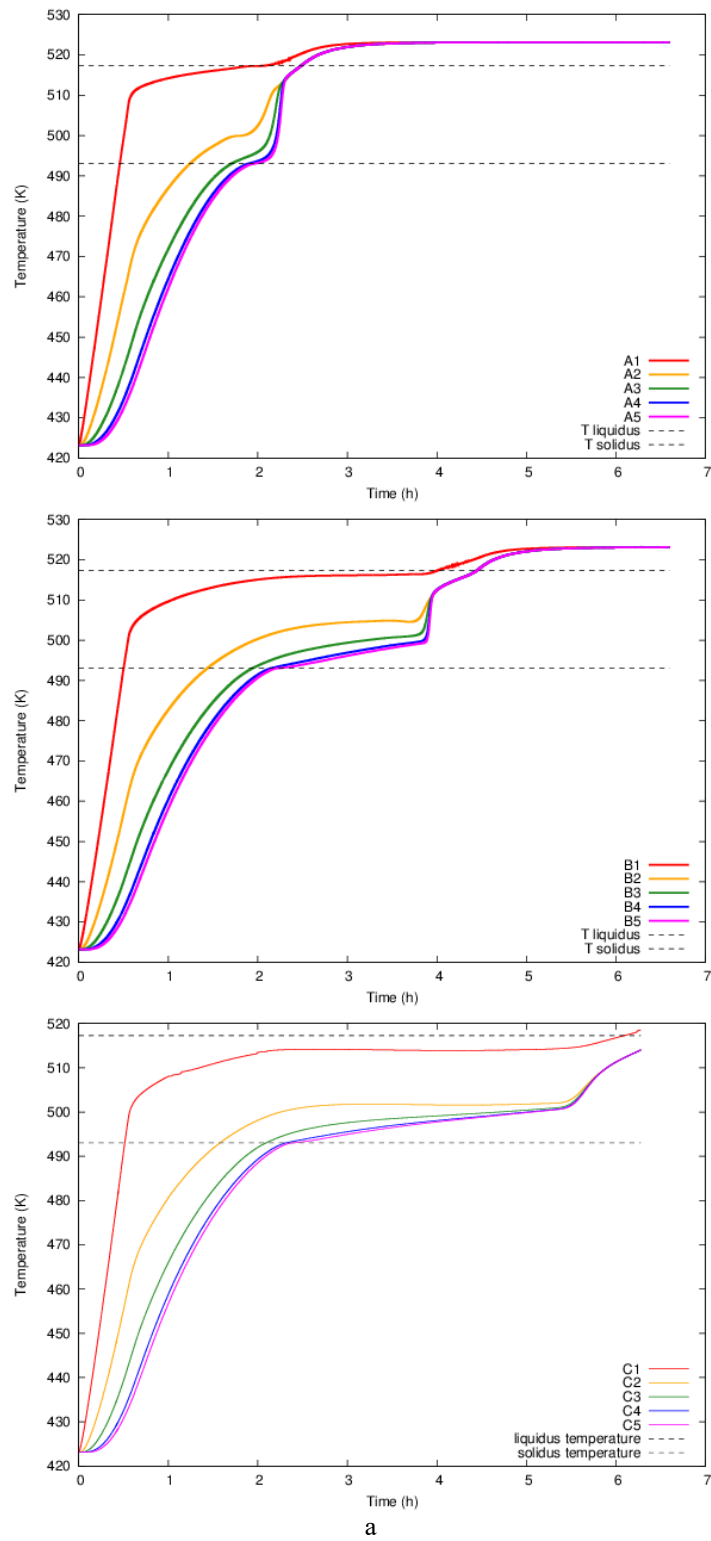
Figure 10 - Time series of temperature in the monitored points
