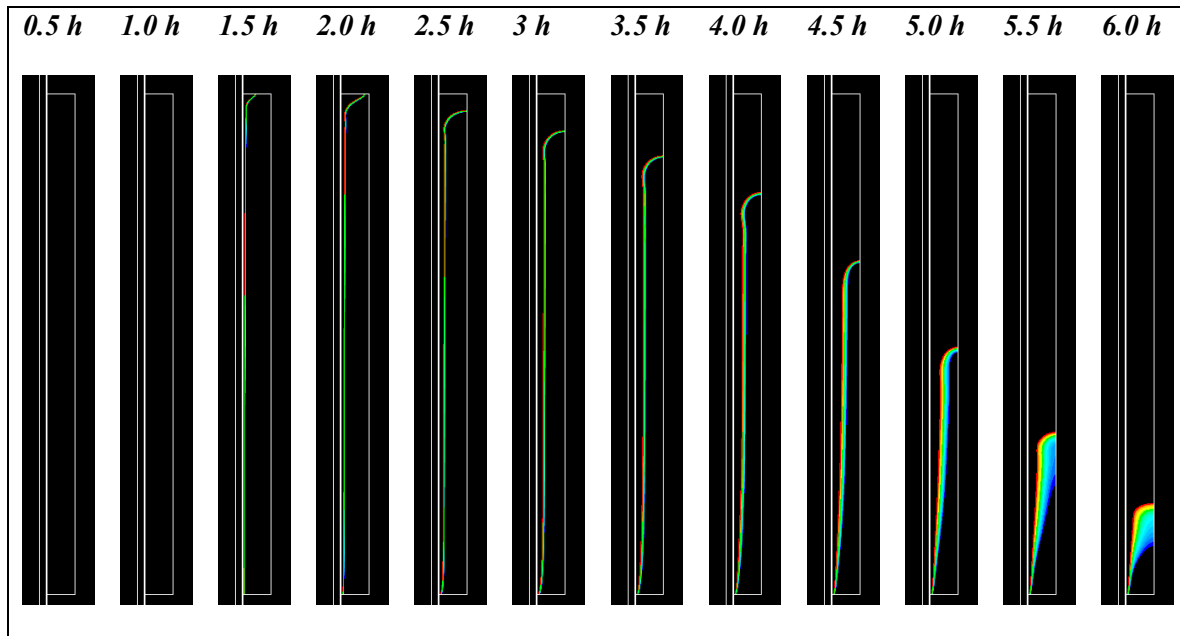
Figure 9 – Position of the melting front every 30 min
