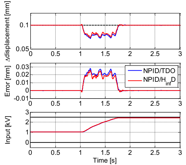
Fig. 19. Disturbance rejection comparison, experimental results, NPID / TDO (1.77 kV) and NPID / H ∞ D (1.77 kV).
