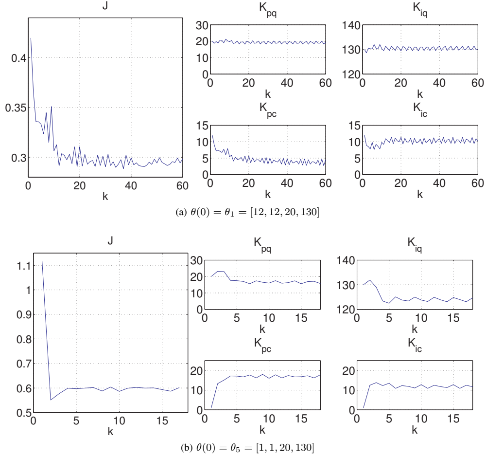
Figure 6. Evolution of J(\theta(k)) and \theta(k)
