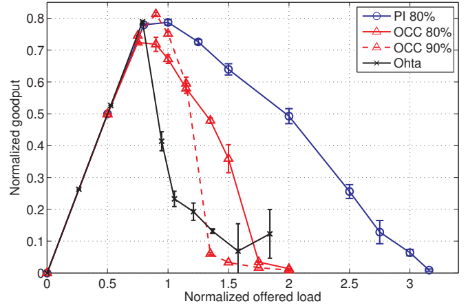
Figure 11. Goodput comparison
