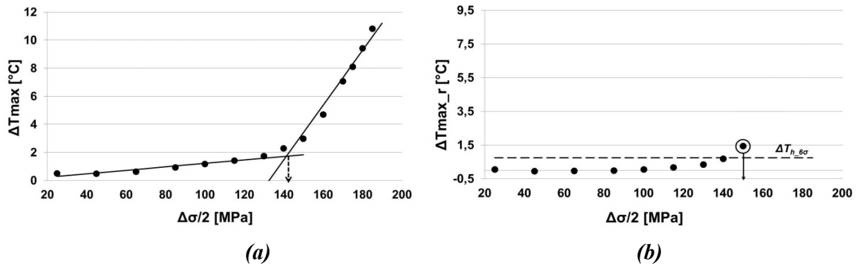
Figure 7. Fatigue limit evaluation: (a) Comparison between Luong's method and (b) proposed method, ASTM A 182 grade F6NM, specimen1.
