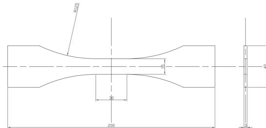
Figure 1. Dimensions (mm) and geometry of specimens
