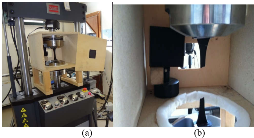
Figure 2. (a) Loading machine, insulated chamber, specimen (b) Inside of insulated chamber: specimen, black body and IR camera.
