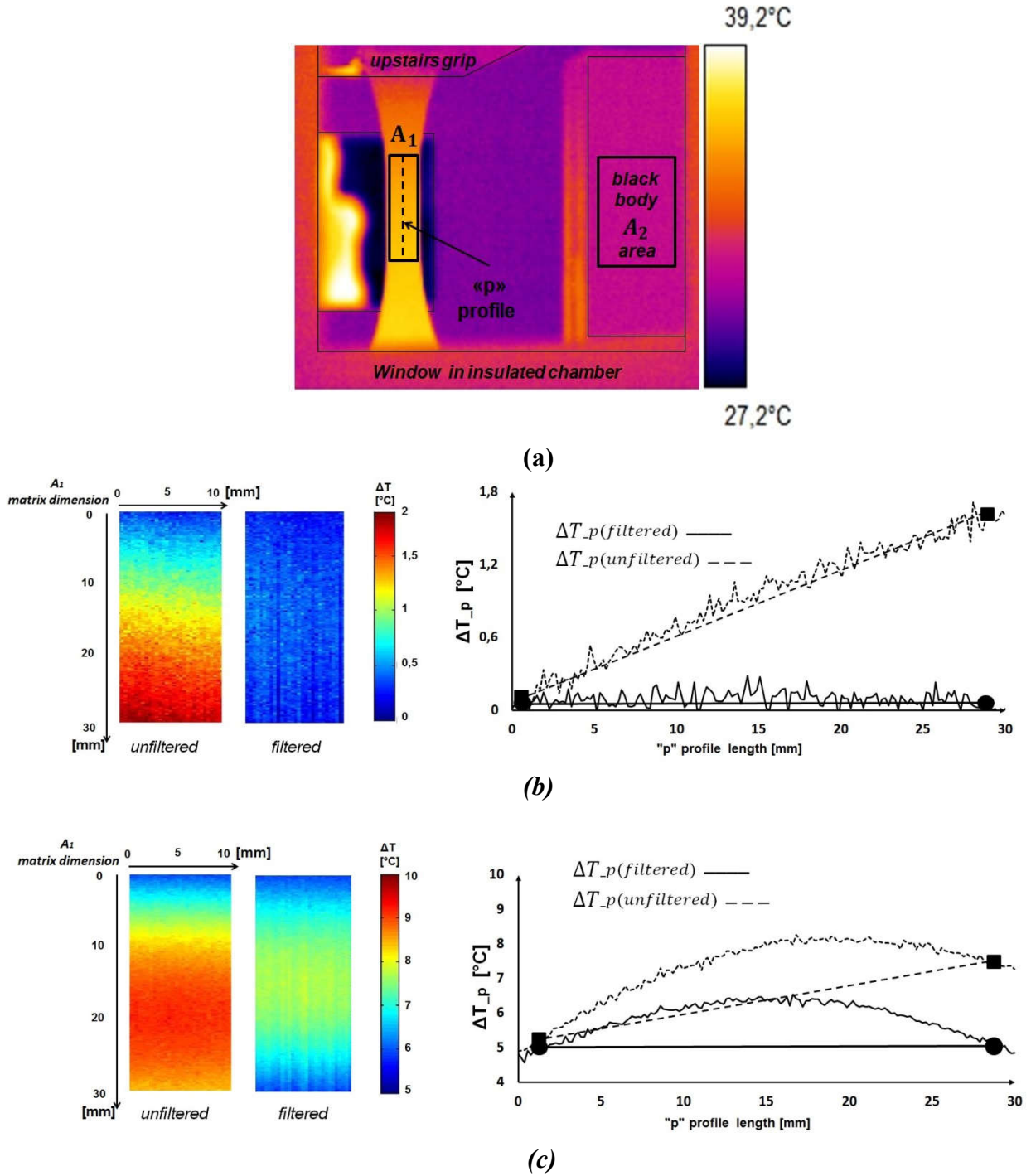
Figure 4. a) Areas and thermal profile “p” considered for analysis (ASTM A182, specimen 1): b) temperature trend along “p” profile at load step 8 (140 MPa), c) temperature trend along “p” profile at load step 13 (180 MPa).
