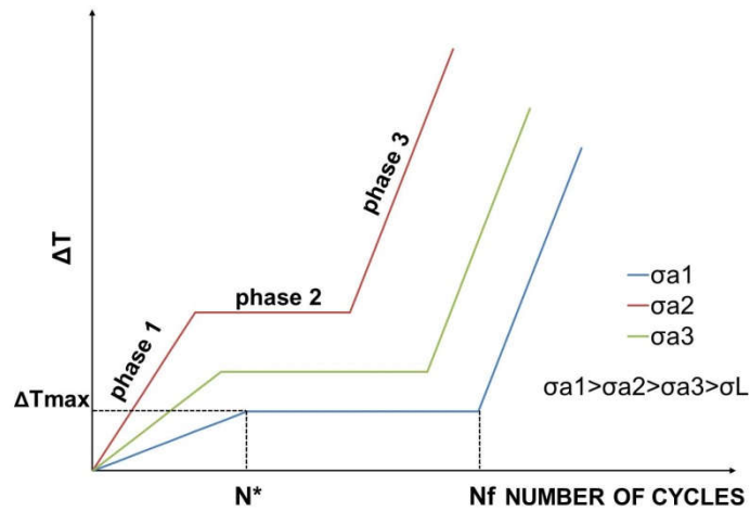
Figure 3. Expected temperature trend during a fatigue test at different load stress values above fatigue limit.
