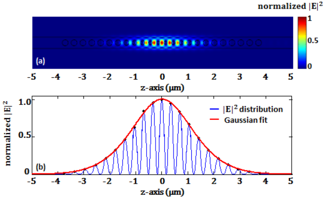
Fig. 3. (a) Distribution of |E|^2 in the PhC dielectric cavity with R_1 = 70 nm and \Lambda_1 = 330 nm, N = 5 and N_l = 6 at resonance \lambda_R = 1589.54 nm; (b) Comparison between the distribution of |E|^2 (blue line) and a Gaussian fit (red line).
