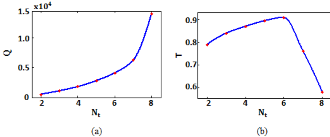
Fig. 5. (a) Q-factor; and (b) resonance transmission behavior as a function of N_t .
