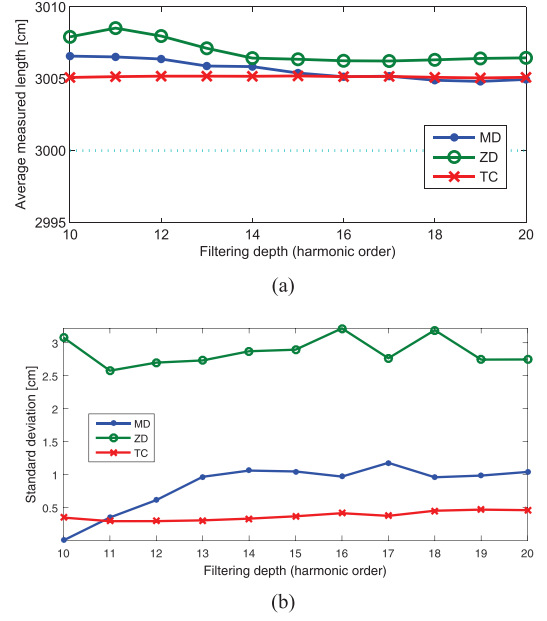
Fig. 8. Repeatability analysis for a 30-m-long cable in terms of average measured length (a) and standard deviation (b).
