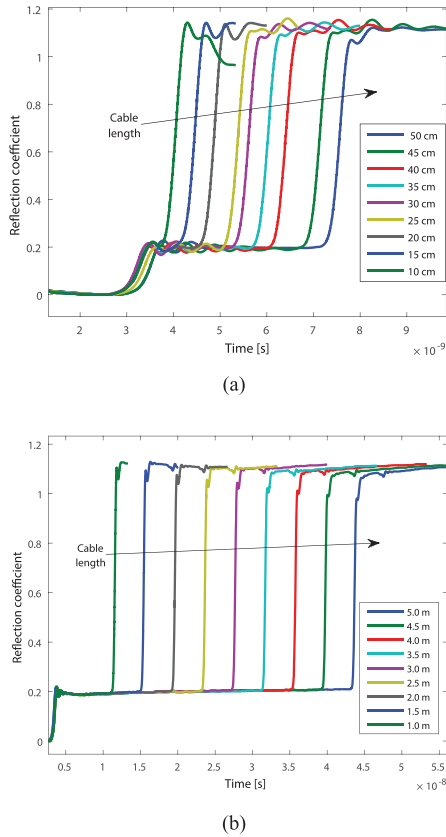
Fig. 5. Measured reflectograms for cable lengths from (a) 10 to 50 cm and (b) 1 to 5 m.
