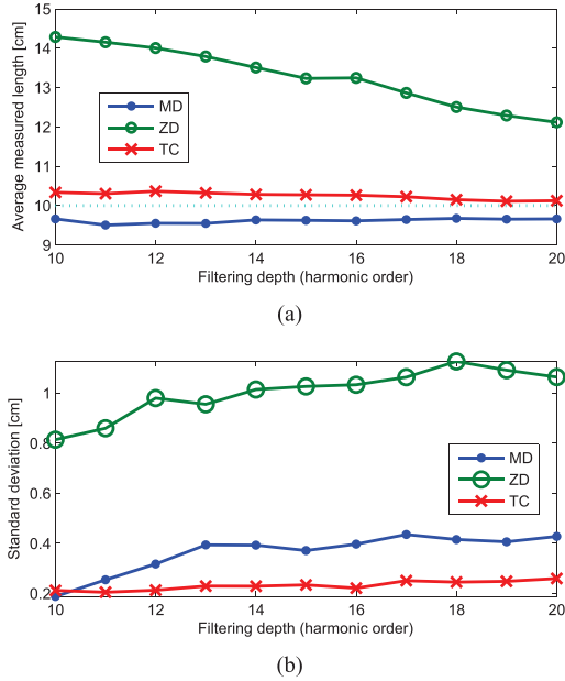
Fig. 7. Repeatability analysis for a 10-cm-long cable in terms of average measured length (a) and standard deviation (b).
