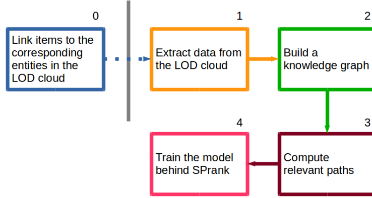
Fig. 2. A schematic representation of the SPrank approach.
