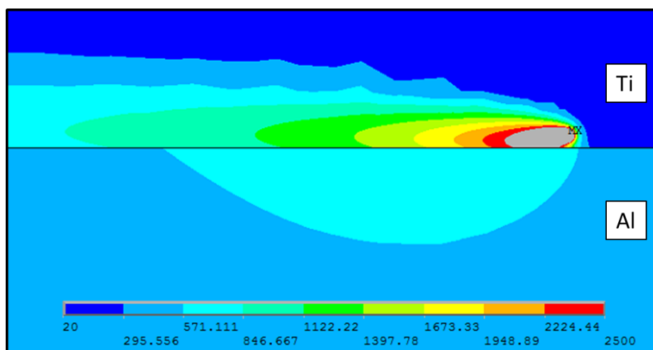
Fig.14 Temperature fields on the top surface of the Al-Ti joint
