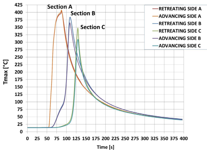
Figure 7. Thermal profiles on the advancing and retreating side acquired by thermocouples placed at 21 mm from the central line of joint (test n. 1 , n = 500 RPM; v = 20 cm/min) in correspondence with three sections of the welding.
