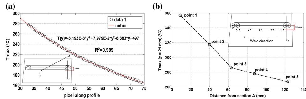
Figure 11. Thermal profile along the y axis and the best fit of data obtained with a cubic equation (a), T_{max} trend along the weld direction (b).
