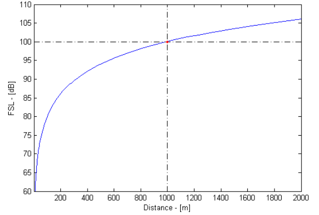
Fig. 11. Free Space Loss vs. Transmitting distance (carrier frequency is 2.4 GHz)
