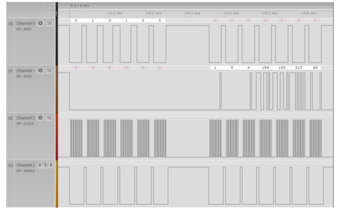
Fig. 4. SPI Query and response of Temperature channel using Salae Logic Analyzer; Trigger command has been sent before time zero and therefore it's not visible
