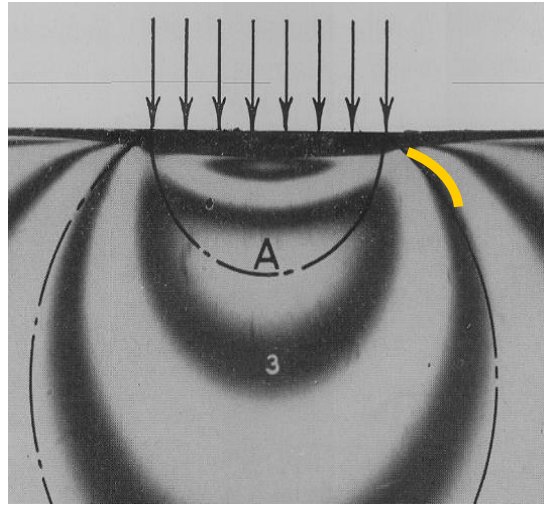
Figure 20. Photoelastic pattern of an infinite plate under a uniform load [31]
