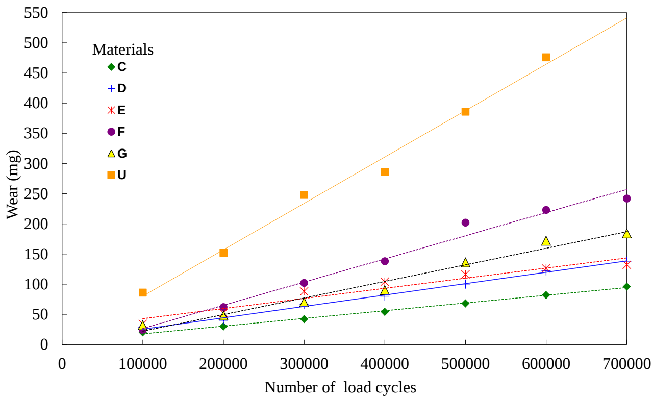
Figure 7. Effect of fatigue cycles on wheel wear
