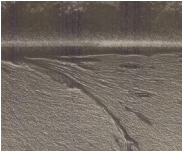
Figure 1. Fracture pattern on the actual railroad wheel
