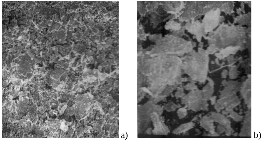
Figure 22. SEM pictures (100X) of wear particles from test facility (a) and actual railroad (b)
