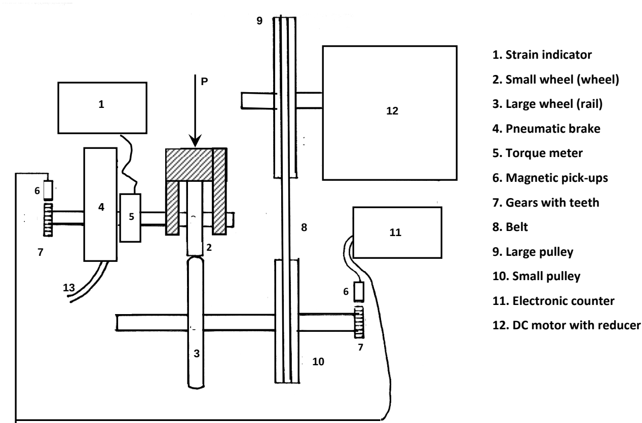
Figure 2. Schematic of the testing apparatus used to simulate the rail-wheel rolling contact
