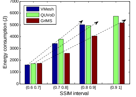
Fig. 21. Energy consumption vs. SSIM intervals
