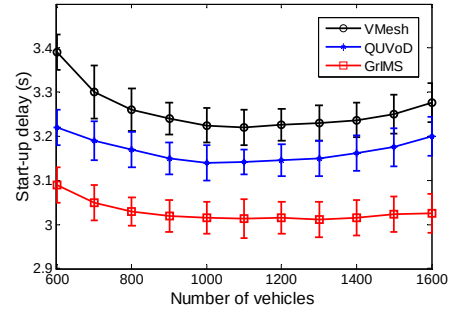
Fig. 11. Start-up delay vs. Number of vehicles
