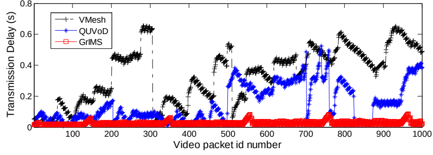
Fig. 8. Packet transmission delay during a video transmitting procedure
