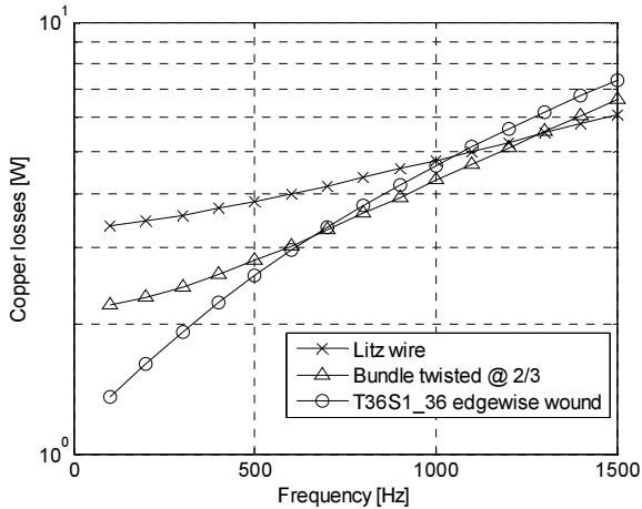
Fig. 17. U-core. Comparison of the losses obtained using the proposed optimal twisting strategy with those obtained with state-of-the-art commercial Litz wire.
