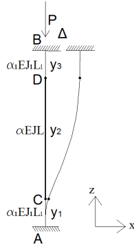
Figure 21. Sketch of the considered structure.
