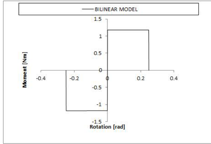
Figure 10. Moment-Rotation relationship of non-linear link.
