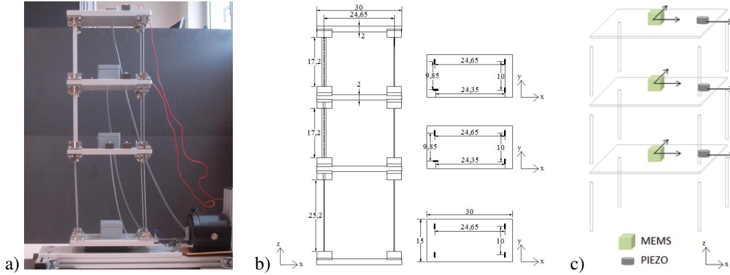
Figure 2. a) Experimental model; b) Schematic drawing; c) Lay out of sensors and measuring direction.
