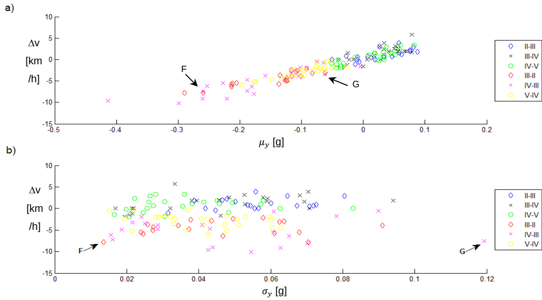
Figure 8 Vehicle speed variation versus a) mean \mu_y and b) standard deviation of acceleration on y-axis, \sigma_y
