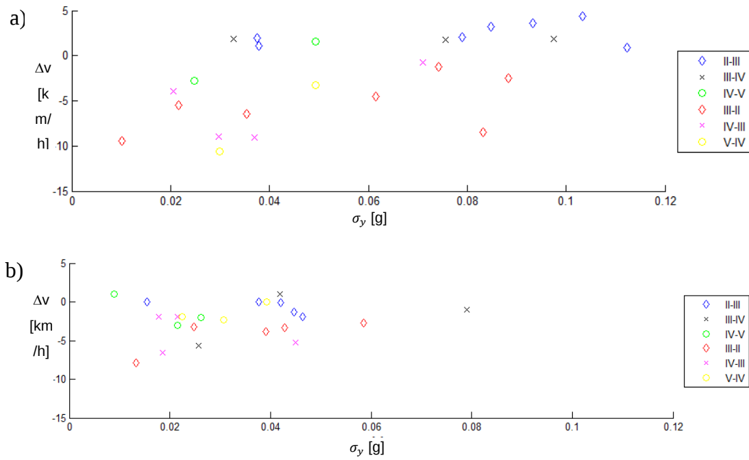
Figure 13 Comparison of vehicle speed variation \Delta v versus standard deviation of acceleration \sigma_y for a) driver A and b) driver B.
