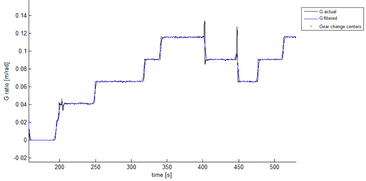
Figure 5 Actual G(t) and its filtered version G_f(t) . The red markers represent the reference points for transition analysis.
