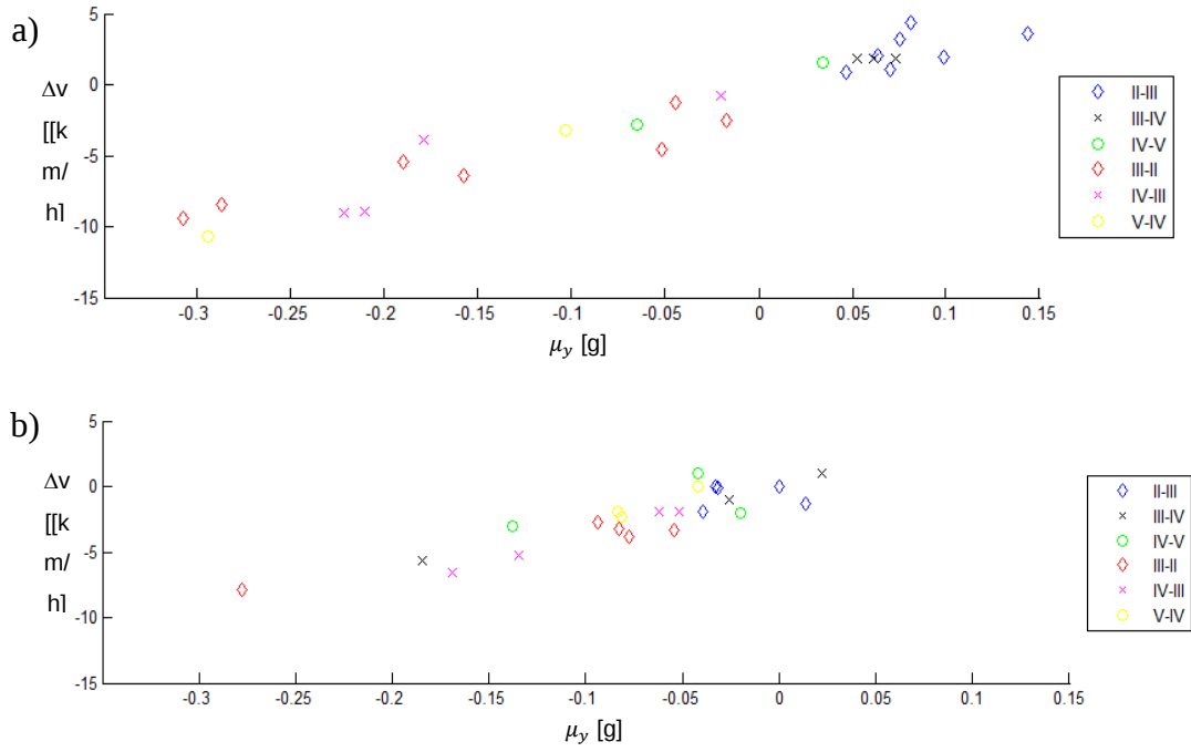
Figure 12 Comparison of vehicle speed variation \Delta v versus mean acceleration \mu for a) driver A and b) driver B.
