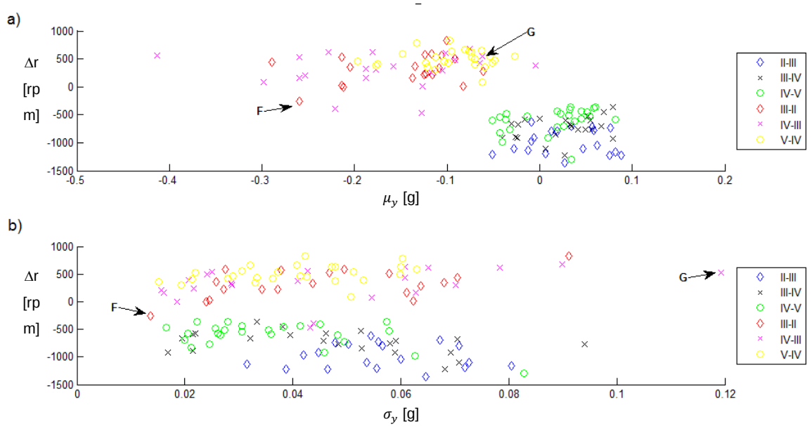
Figure 7 Engine speed variation versus (a) mean and (b) standard deviation of acceleration on y-axis
