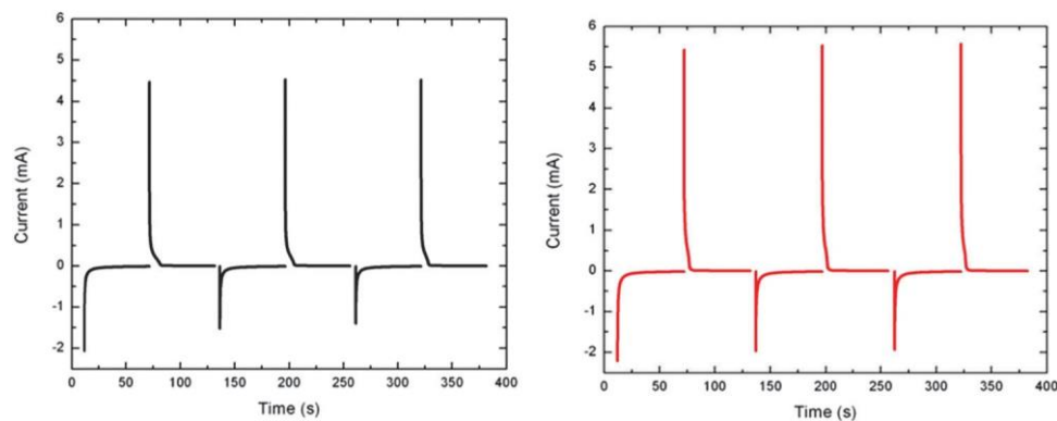
Fig. 4 Chronoamperometric measurements for Sample A (left hand side) and Sample B (right hand side).
