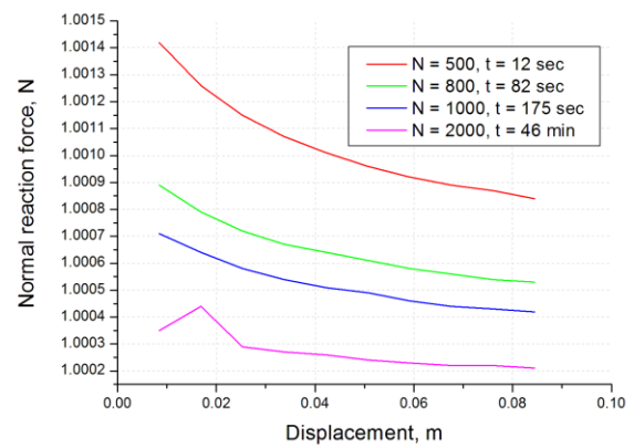
Fig. 4 The profiles of worn parabolic indenter (a) and normal reaction force (b) versus tangential displacement, obtained for different numbers of spatial steps in the simulated region.
