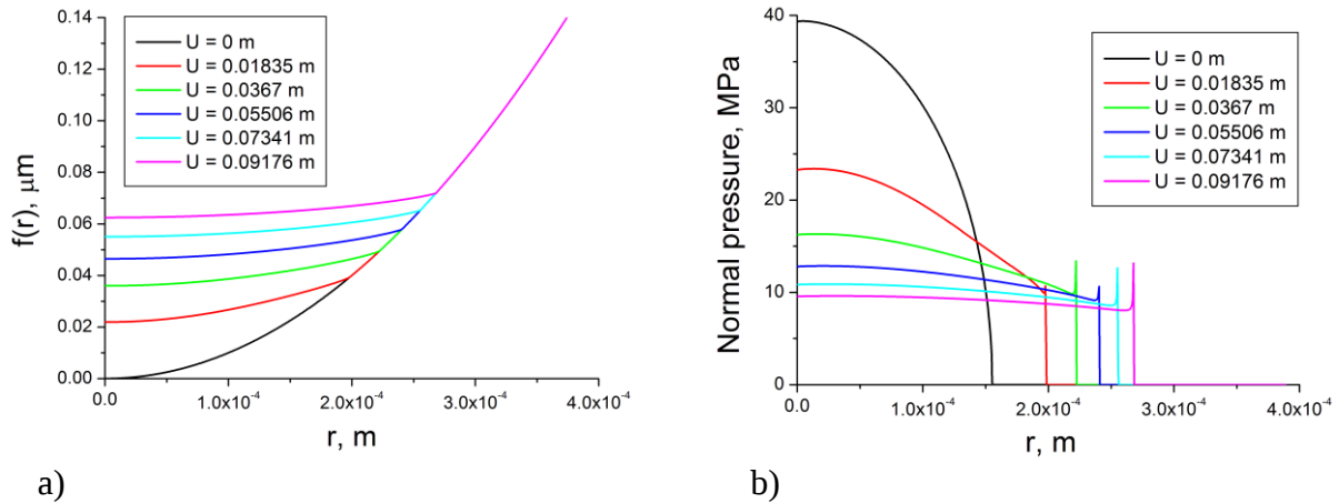
Fig. 2 Profiles of worn indenter (a) and normal pressure distributions (b) obtained in the presented model and in three-dimensional FEM model and MDR-based model. [V1]
