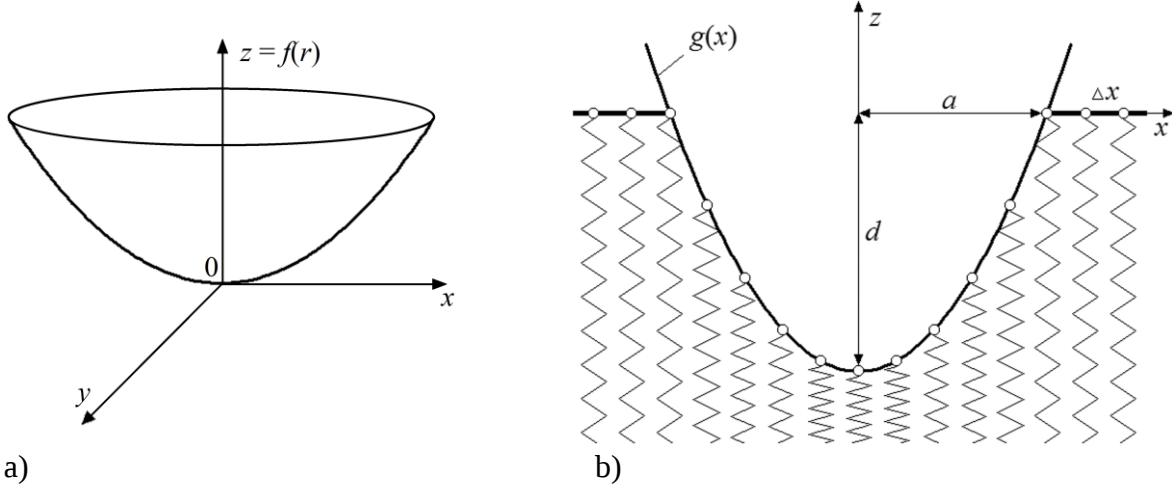
Fig. 1. The 3-dimensional body of revolution (a); and the corresponding one-dimensional MDR-transformed profile in a contact with the elastic foundation.
