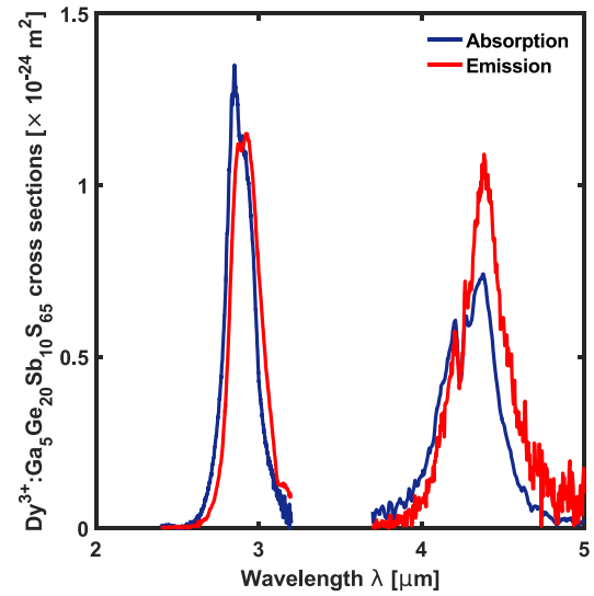
Fig. 3. Calculated emission and absorption cross-sections for the \text{Dy}^{3+}:\text{Ga}_5\text{Ge}_{20}\text{Sb}_{10}\text{S}_{65} glass.
