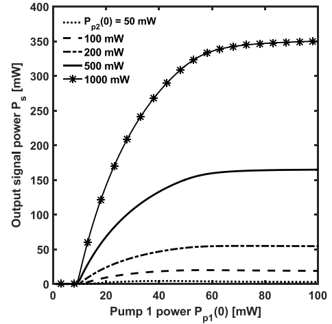
Fig. 5. Optical signal power P_s of the \text{Dy}^{3+} -doped PCF laser, versus the input pump #1 power P_{p1}(0) at the wavelength \lambda_{p1} = 2850 \text{ nm} for different input pump #2 powers at the wavelength \lambda_{p2} = 4092 \text{ nm} , P_{p2}(0) = 50 \text{ mW} (dotted curve), P_{p2}(0) = 100 \text{ mW} (dashed curve), P_{p2}(0) = 200 \text{ mW} (dash-dot curve), P_{p2}(0) = 500 \text{ mW} (solid curve), P_{p2}(0) = 1000 \text{ mW} (solid curve with asterisk markers). Optical cavity length L = 0.5 \text{ m} ; dopant concentration N_{\text{Dy}} = 4 \times 10^{25} \text{ ions/m}^3 ; first mirror reflectivity R_1 = 99\% ; second mirror reflectivity R_2 = 30\% .
