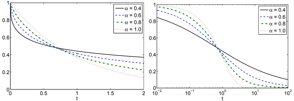
FIGURE 2. Relaxation function \Psi_{CC}(t) on varying \alpha .
