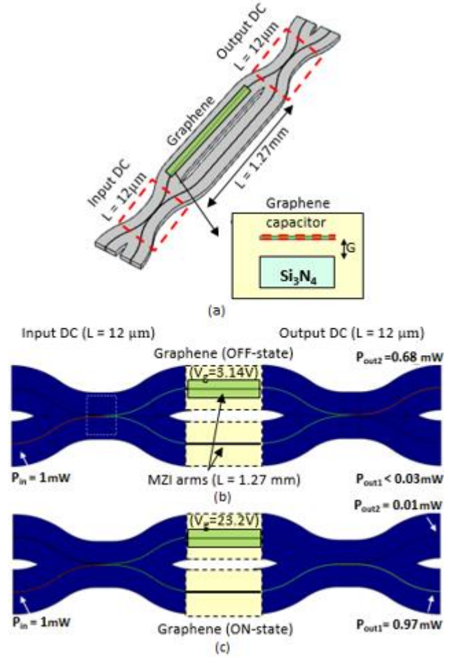
Fig. 3. (a) Configuration of the graphene-based MZI switch; the inset shows the graphene capacitor placed above the \text{Si}_3\text{N}_4 waveguide, with G = 240 nm. (b) 2D FEM simulations of the graphene-based MZI in OFF-state with V_g = 3.14 V; (c) in ON-state with V_g = 23.2 V.
