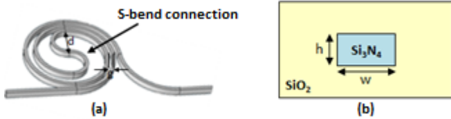
Fig. 2. (a) Spiral waveguide configuration with a length L , a diameter of S-bend connection d = 200 \mu\text{m} and a separation between neighboring waveguides g = 3 \mu\text{m} . (b) Cross-section of the \text{Si}_3\text{N}_4 waveguide
