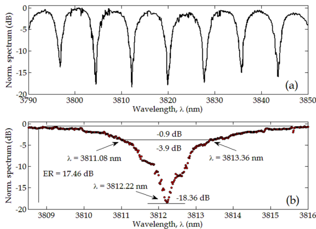
Fig. 5. (a) Ge-on-Si add-drop racetrack resonator spectrum. (b) A quality factor, Q , of \sim 1,700 can be seen.
