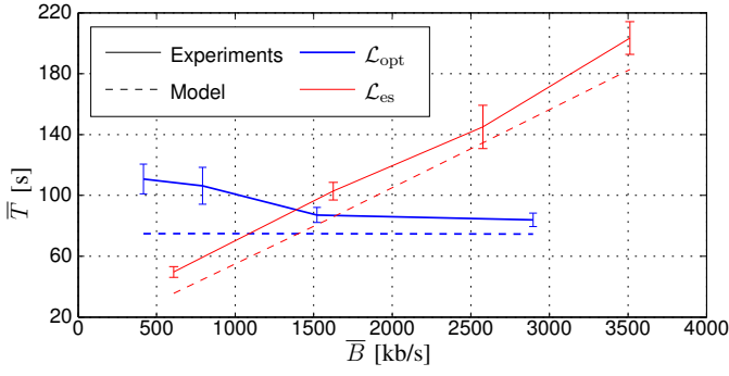
Fig. 10. Comparison between the video level switching period obtained with optimal level set \mathcal{L}_{\text{opt}} = \{300, 573, 1094, 2090, 4000\} kb/s or with equally spaced levels \mathcal{L}_{\text{es}} = \{300, 1225, 2150, 3075, 4000\} kb/s as a function of \bar{B}
