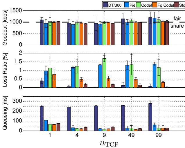
Figure 7: A single GCC flow with n_{TCP} concurrent TCP flows
