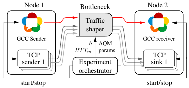
Figure 3: Experimental testbed
