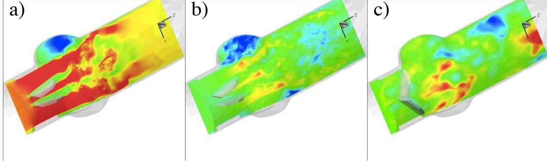
Figure 5. Instantaneous snapshots of axial velocity through a central symmetry plane at three instants of the cycle for the Newtonian fluid model: a) peak flow, b) valve closing and c) flow settling. (red maximum values, blue minimum values).
