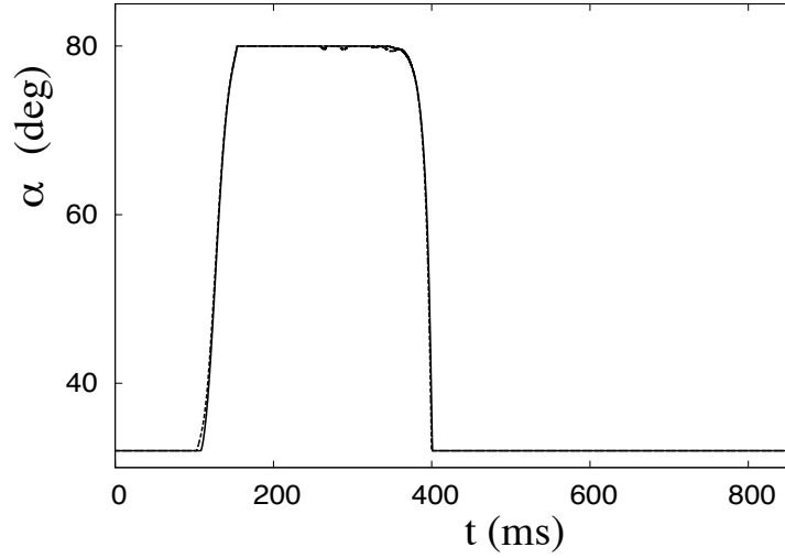
Figure 6. Angular position of the upper leaflet of the mechanical valve during the flow cycle: solid line for the Newtonian fluid model, dashed line for the non-Newtonian fluid model.
