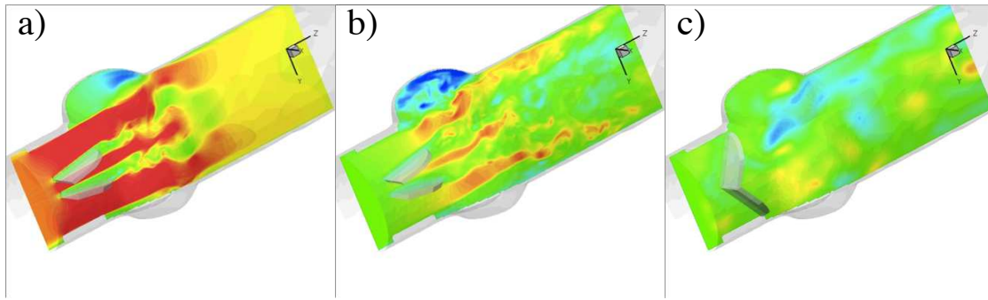
Figure 10. Instantaneous snapshots of axial velocity through a central symmetry plane at three instants of the cycle for the non-Newtonian fluid model: a) peak flow, b) valve closing and c) flow settling. (red maximum values, blue minimum values).
