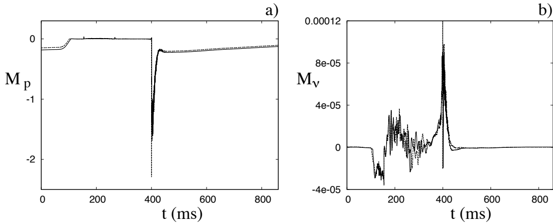
Figure 7. Time evolution of the pressure (a) and viscous (b) moments about the hinge for the upper leaflet of the mechanical valve during the flow cycle: solid line for the Newtonian fluid model, dashed line for the non-Newtonian fluid model.
