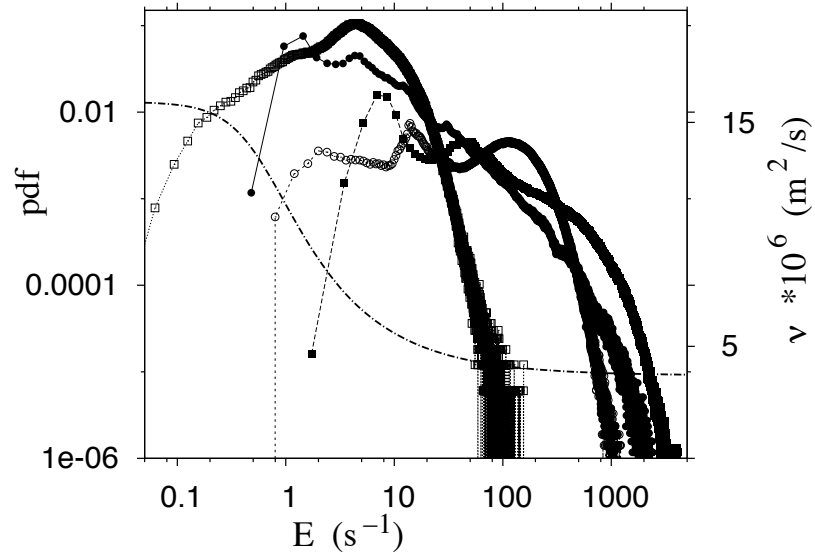
Figure 9. Probability distribution functions of the shear rate for 4 representative instants in the cycle for the non-Newtonian fluid model. The pdfs are overlaid onto a curve for the shear rate dependence of the blood viscosity (hematocrit 40%). Symbols as in Figure 2.
