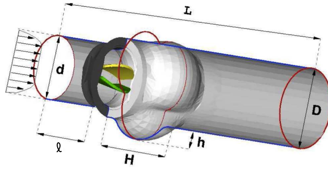
Figure 1. Sketch of the computational set-up. Main lengths: D = 1.26d , \ell = d , L = 5d , H = 1.14d , h = 0.26d .
