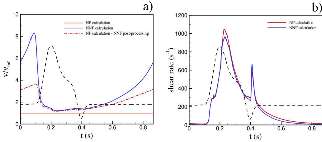
Figure 12. a) Time evolution of the averaged viscosity felt by the fluid particles for the non-Newtonian fluid (NNF) model (solid blue), the Newtonian fluid (NF) model (solid red) and NF simulation with NNF calculation of haemolysis (chaindot red). b) Averaged equivalent shear-rate experienced by the fluid particles for the non-Newtonian fluid (NNF) model (solid blue) and the Newtonian fluid (NF) model (solid red).
