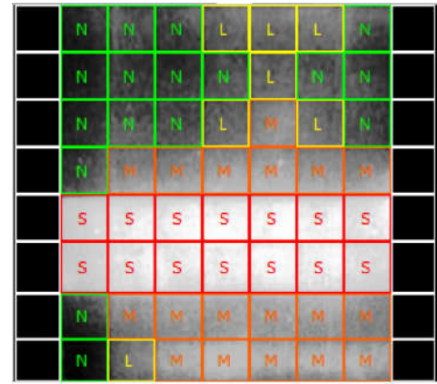
Fig. 4. Non-uniform (masked in black) cells; Normal (green N) cells; Light (yellow L), medium (orange M) and strong (red S) hot cells.
