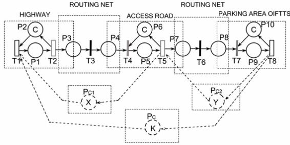
Fig. 10. Example of TPN model of IFTT.
