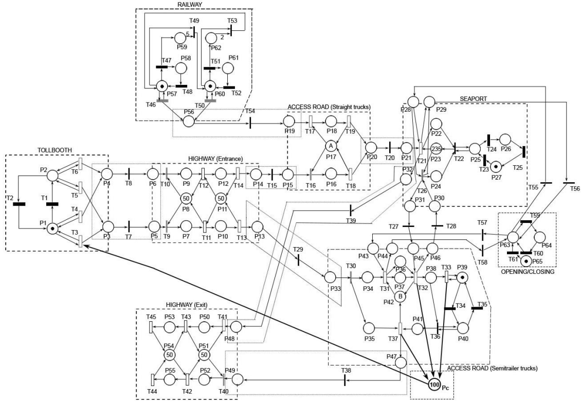
Fig. 13. TPN model of the literature example in Fig. 12 [23].
