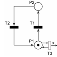
Fig. 4a. Railway subnet model: only incoming ITUs.
