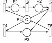
Fig. 8. Customs area subnet model.
