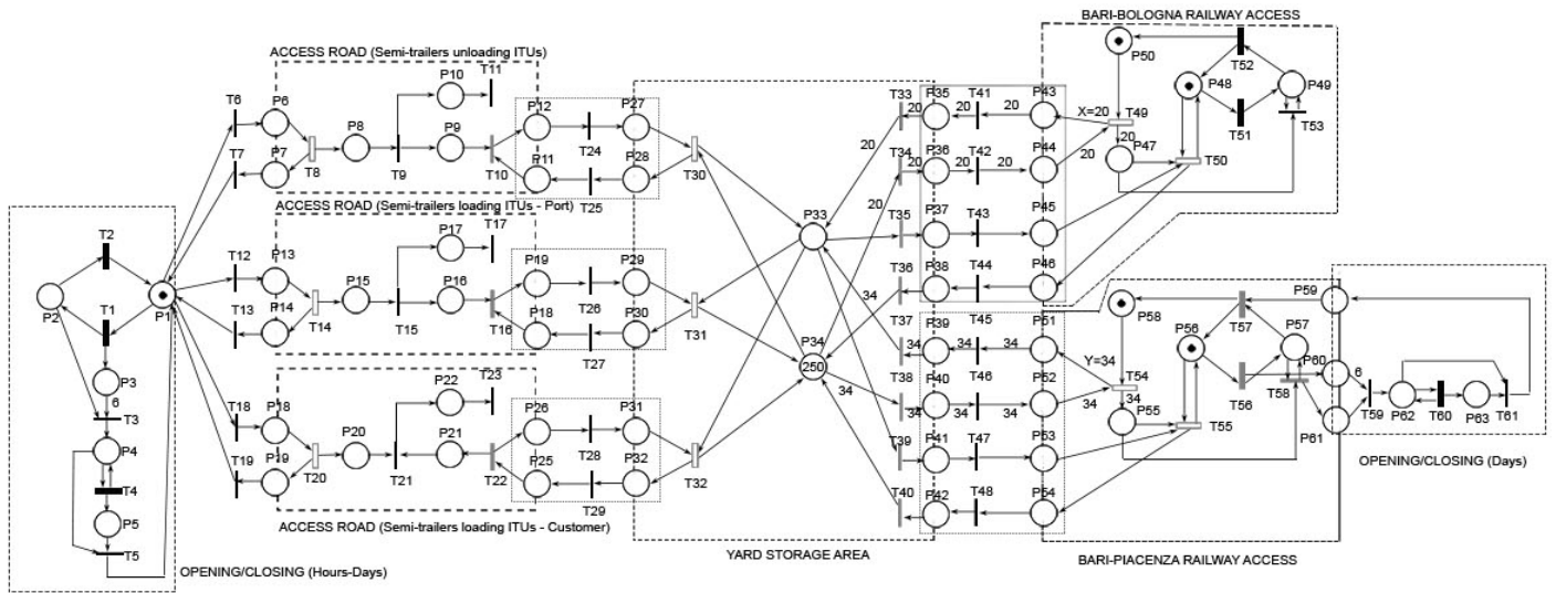
Fig. 15. TPN model of the real case study in Fig. 14.
