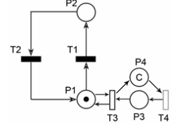
Fig. 4b. Railway subnet model: incoming and outgoing ITUs.
