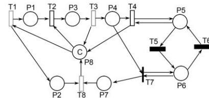
Fig. 6b. Access road subnet model for semi-trailer trucks with reassembly.
