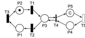
Fig. 5. Seaport, river port or airport subnet model.
