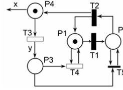
Fig. 4c. Railway subnet model: incoming and outgoing ITUs with separate load/unload.
