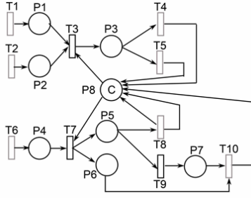
Fig. 8. Customs area subnet model.
