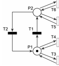
Fig. 2. Highway portion subnet model.
