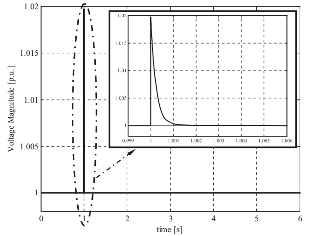
Fig. 7. Time domain behavior of the voltage at the control bus (bus no. #11).
